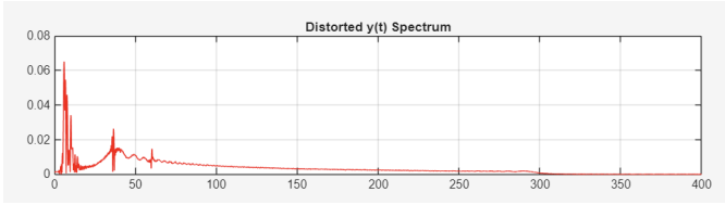
Figure 6. Magnitude Spectrum of the Distorted Signal y(t) .
