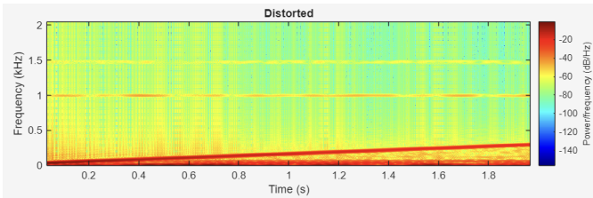
Figure 7. Distorted Signal y(t) Spectrogram Frequency Sweep.
