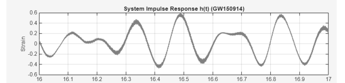
Figure 4. 16-17s Merger Window of the GW150914 Impulse Response h(t) in the Time-Domain.
